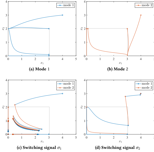
Figure 1: Trajectories of the switched system (37) for (a) mode 1 with initial states (4, 3), (3, 2), (3, 0.1), and (3, 0); (b) mode 2 with initial states (4, 3), (3, 2), (0.1, 2), and (0, 2); (c) switching signal \sigma_1 with initial states (4, 3), (3, 0), (0, 2), and (0, 0); (d) switching signal \sigma_2 with initial state (4, 3). The circles mark the beginning of segments after switching. The gray rectangle represents \Omega = [0, 3.04] \times [0, 2.03] .
